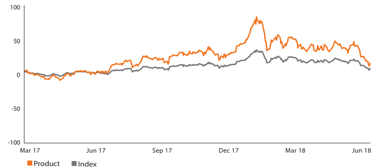
Cumulative performance (%)
